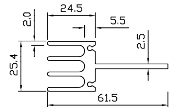
SP 5104 WT – 1.015 KG/M PERIMETER – 291.362 MM
