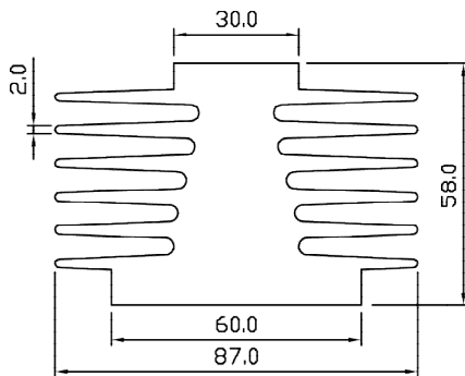
SP 8035 WT – 7.779 KG/M PERIMETER – 870.206 MM
