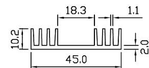
SP 5026 WT – 0.473 KG/M PERIMETER – 222.058 MM
