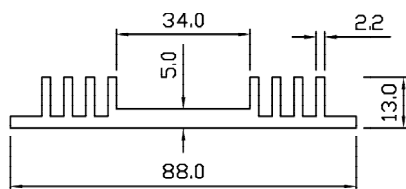
SP 5037 WT – 1.371 KG/M PERIMETER – 338.00 MM
