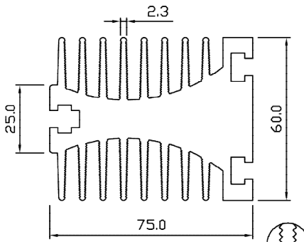
SP 7104 WT – 6.772 KG/M PERIMETER – 1184.330 MM
