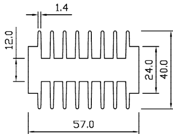
SP 5050 WT – 3.198 KG/M PERIMETER – 568.223 MM
