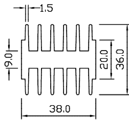
SP 5035 WT – 1.760 KG/M PERIMETER – 404.183 MM
