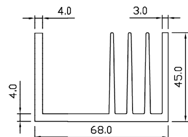
SP 6564 WT – 2.251 KG/M PERIMETER – 546.367 MM
