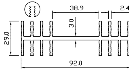
SP 5007 WT – 1.808 KG/M PERIMETER – 780.798 MM
