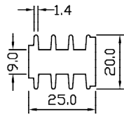
SP 5003 WT – 0.861 KG/M PERIMETER – 147.460 MM
