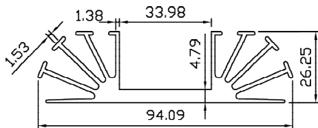
SP 7463 WT – 1.716 KG/M PERIMETER – 575.592 MM
