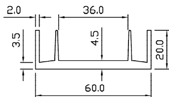
SP 5031 WT – 0.998 KG/M PERIMETER – 252.299 MM
