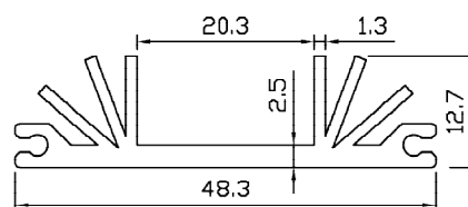
SP 0106 WT – 0.570 KG/M PERIMETER – 240.132 MM
