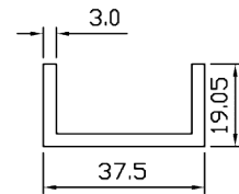
SP 5033 WT – 0.564 KG/M PERIMETER – 145.200 MM
