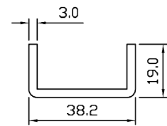
SP 5030 WT – 0.558 KG/M PERIMETER – 143.824 MM
