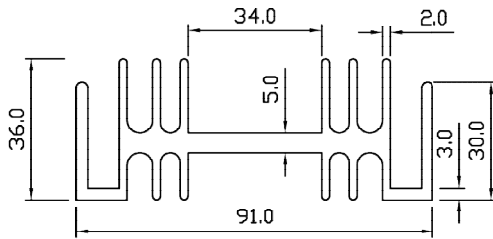
SP 5036 WT – 2.612 KG/M PERIMETER – 641.097 MM
