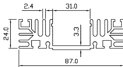
SP 5048 WT – 2.126 KG/M PERIMETER – 617.949 MM
