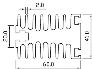
SP 6807 WT – 3.591 KG/M PERIMETER – 598.698 MM
