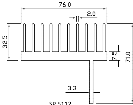
SP 5112 WT – 3.220 KG/M PERIMETER – 735.416 MM
