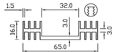
SP 5029 WT – 0.871 KG/M PERIMETER – 424.272 MM
