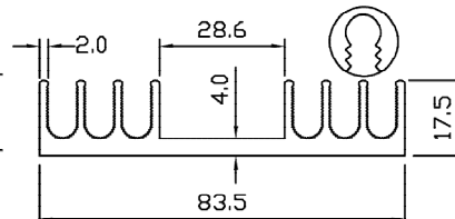
SP 5124 WT – 1.508 KG/M PERIMETER – 434.637 MM
