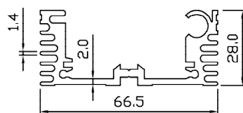
SP 6146 WT – 1.280 KG/M PERIMETER – 426.107 MM
