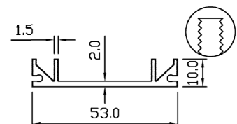
SP 5114 WT – 0.460 KG/M PERIMETER – 209.389 MM
