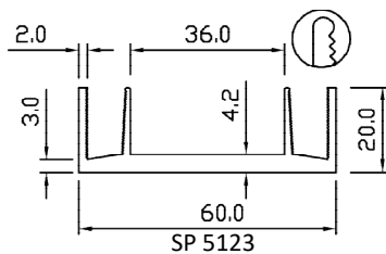
SP 5123 WT – 0.933 KG/M PERIMETER – 281.106 MM
