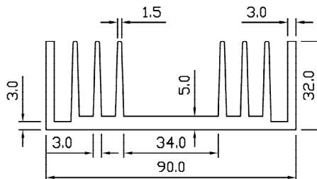
SP 5032 WT – 2.555 KG/M PERIMETER – 617.264 MM
