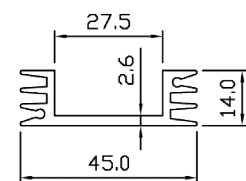
SP 6502 WT – 0.141 KG/M PERIMETER – 104.721 MM
