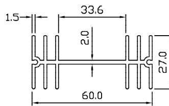
SP 5113 WT – 0.928 KG/M PERIMETER – 422.283 MM
