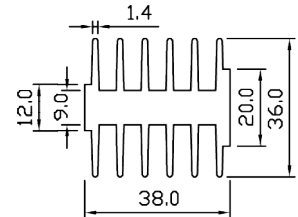
SP 5004 WT – 1.721 KG/M PERIMETER – 404.0 MM
