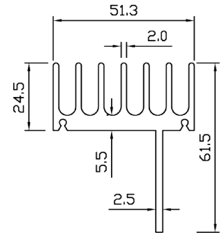
SP 5105 WT – 1.742 KG/M PERIMETER – 446.045 MM
