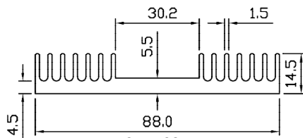
SP 5108 WT – 1.741 KG/M PERIMETER – 438.192 MM
