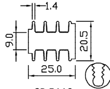
SP 5119 WT – 0.864 KG/M PERIMETER – 182.529 MM
