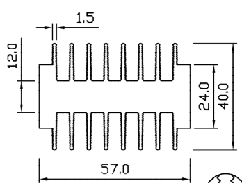
SP 5121 WT – 3.060 KG/M PERIMETER – 745.047 MM
