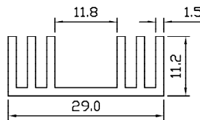
SP 5040 WT – 0.353 KG/M PERIMETER – 177.400 MM
