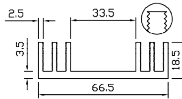
SP 5122 WT – 1.187 KG/M PERIMETER – 568.223 MM
