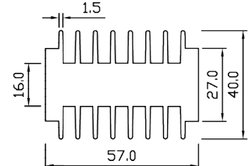
SP 5005 WT – 3.620 KG/M PERIMETER – 513.269 MM
