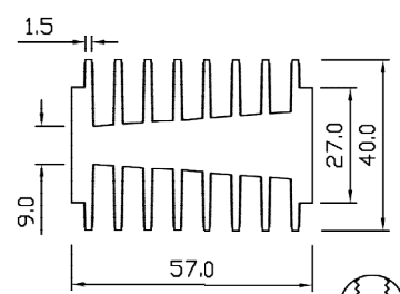
SP 5151 WT – 3.288 KG/M PERIMETER – 731.030 MM
