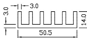
SP 5028 WT – 0.944 KG/M PERIMETER – 239.00 MM
