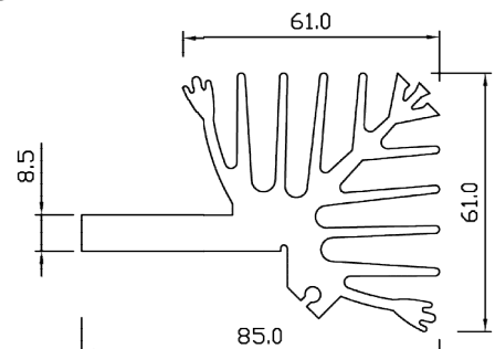
SP 0947 WT – 4.091 KG/M PERIMETER – 753.761 MM
