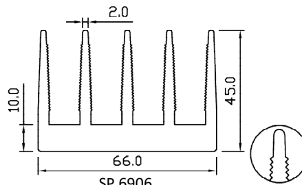
SP 6906 WT – 3.379 KG/M PERIMETER – 569.770 MM
