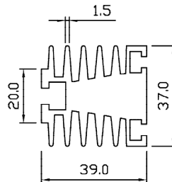
SP 6757 WT – 2.265 KG/M PERIMETER – 422.730 MM
