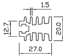
SP 6785 WT – 0.805 KG/M PERIMETER – 201.618 MM
